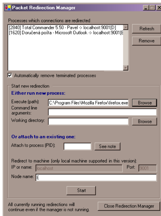
Figure 12: Redirection Manager
