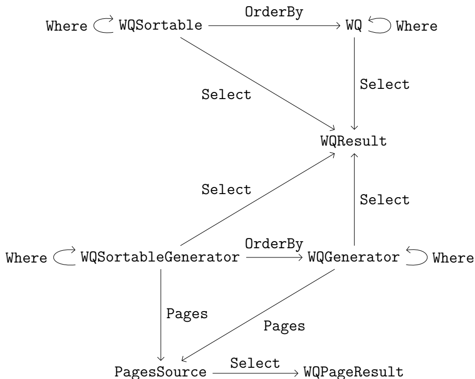
Figure 4.1: State diagram of WikiQuery-related types (WikiQuery is shortened to WQ to save space)
