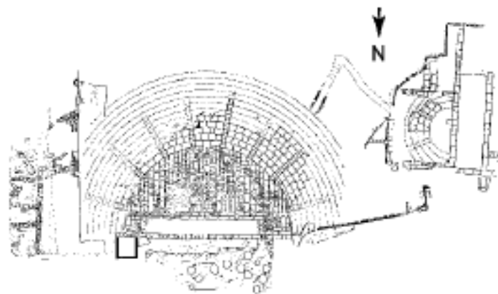
PLAN 103. Acrae, theatre and bouleuterion
