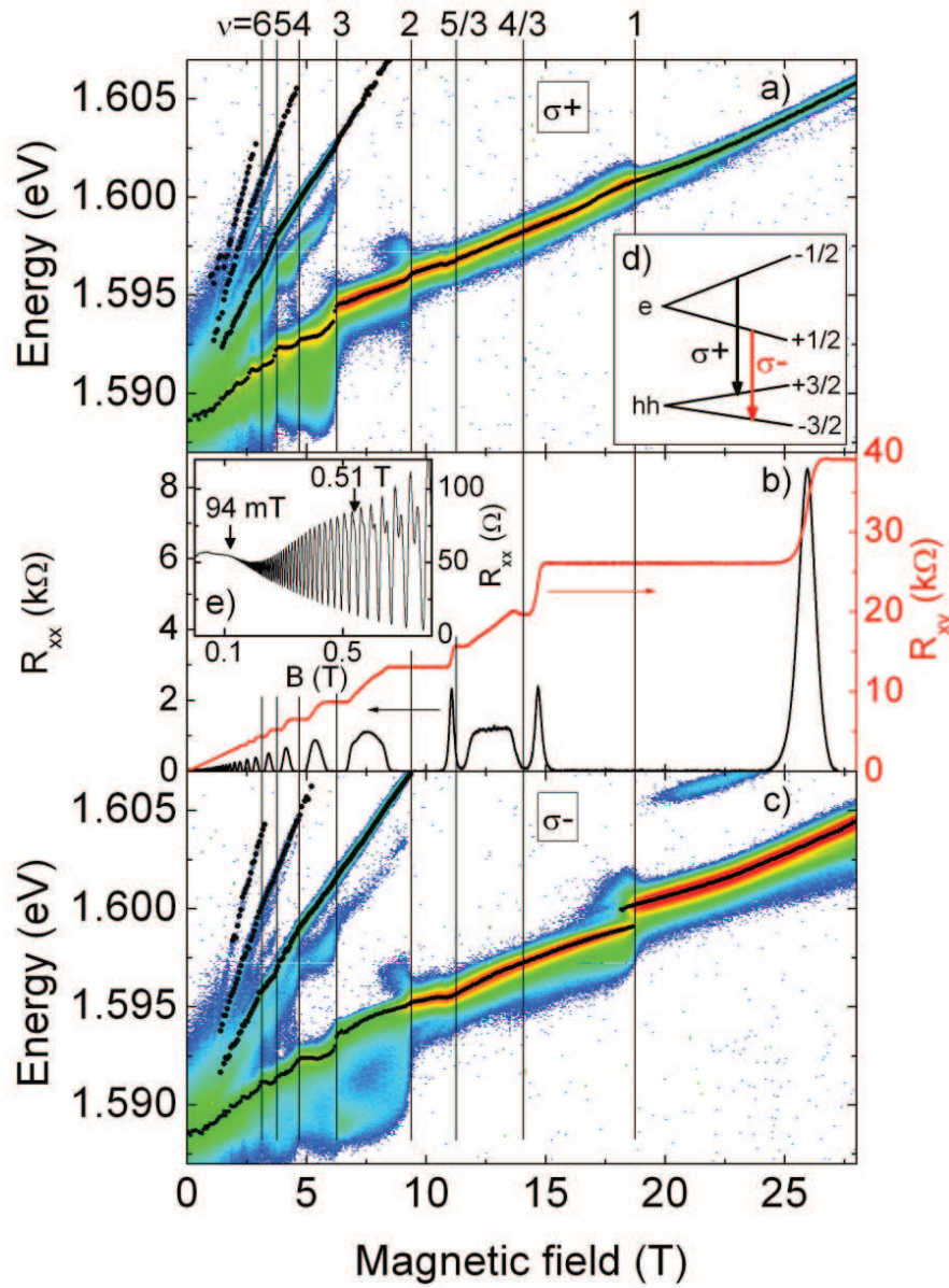
Figure 7.15: (a) and (c) Color plot of \sigma^+ and \sigma^- magneto-PL of a 2DEG in a 20 nm wide CdTe QW, measured at 80 mK, under low power ( \approx 0.5\text{W/m}^2 ), \lambda = 514\text{ nm} -Ar ^+ excitation. Black points indicate the energy of the main peaks. Inset (d) shows the optical selection rules. (b) Results of the simultaneous magneto-transport measurements showing the longitudinal ( R_{xx} ) and Hall ( R_{xy} ) resistance. Vertical lines indicate the Landau level filling factor. Inset (e) shows an expanded view of R_{xx} at low magnetic fields.
