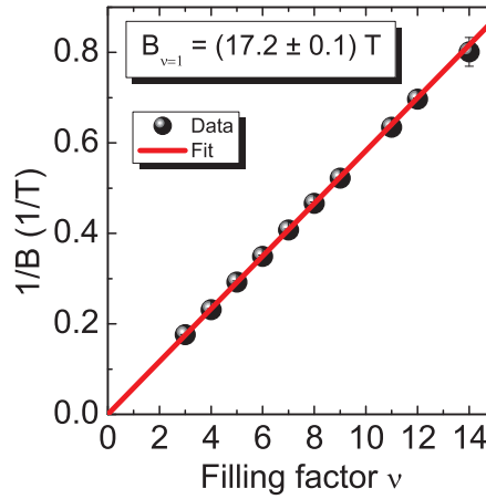
Figure 7.11: Inverse value of the magnetic field versus filling factor to determine concentration of 2DEG. Fitting the slope gives magnetic field at the filling factor \nu = 1 , B_{\nu=1} = 17.2 T and the corresponding electron sheet concentration n_e = 4.2 \times 10^{11} \text{ cm}^{-2} .
