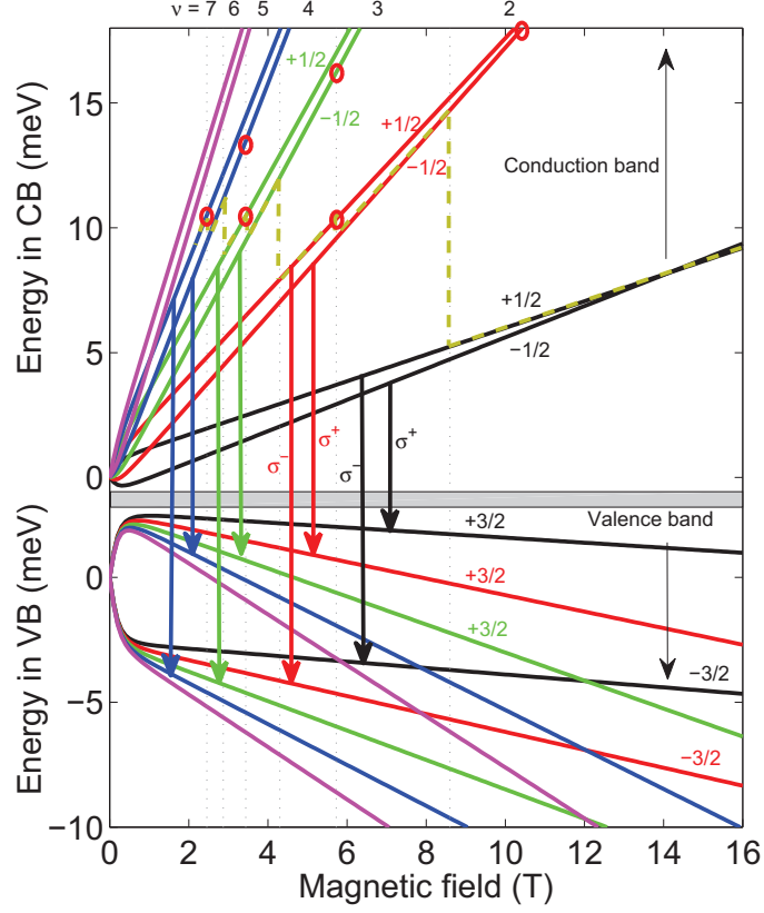
Figure 7.9: Magnetic field evolution of first five electronic (upper curves) and hole (lower curves) Landau levels. Black, red, green, blue and magenta colors correspond to the indices of Landau levels 0, 1, 2, 3 and 4. Arrows depict allowed optical transitions, dotted lines integer filling factors 2, 3, 4, 5, 6 and 7, dark yellow dashed line is a Fermi energy at T = 0 K and red circles show the maximum field up to which the PL emission from a given Landau level was observed.
