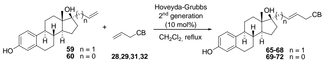
Scheme 35
