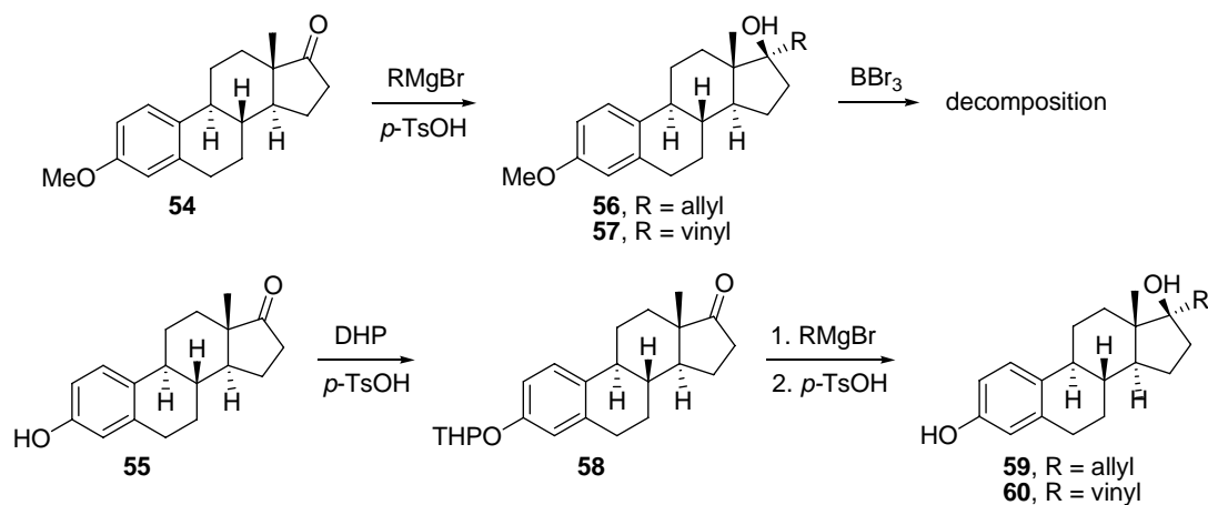
Scheme 33
