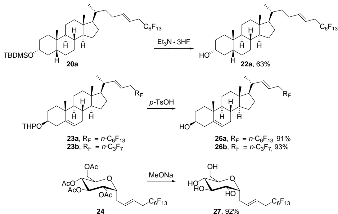
Scheme 28
