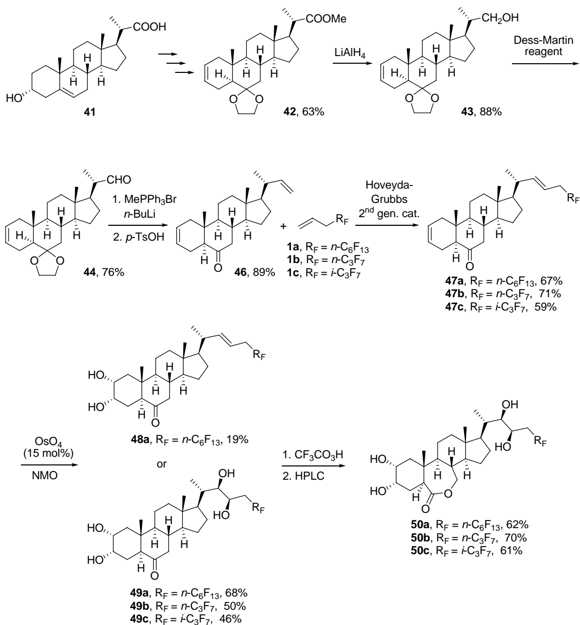
Scheme 32
