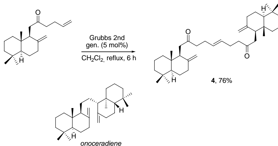
Scheme 8
