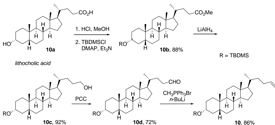
Scheme 26
