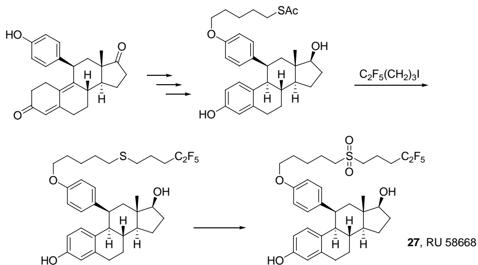
Scheme 20
