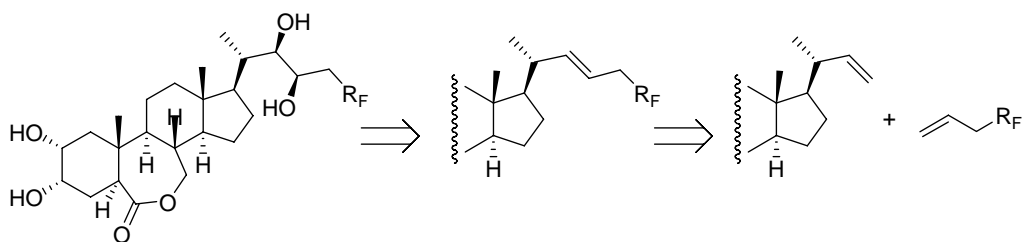
Scheme 31
