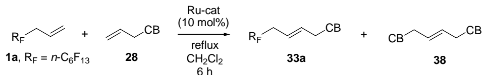
Scheme 30
