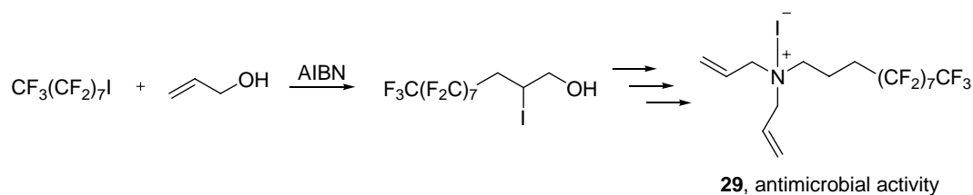
Scheme 22
