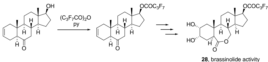
Scheme 21
