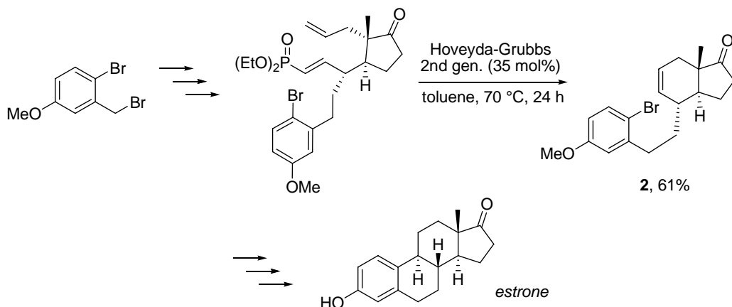
Scheme 6
