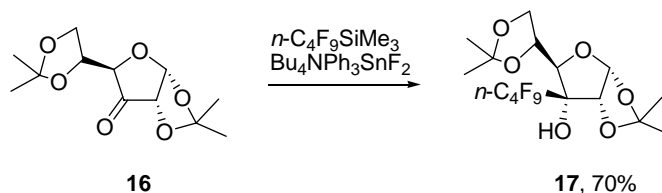
Scheme 15
