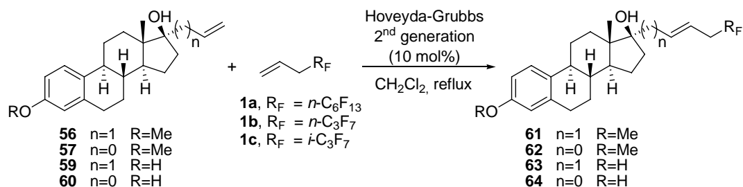
Scheme 34
