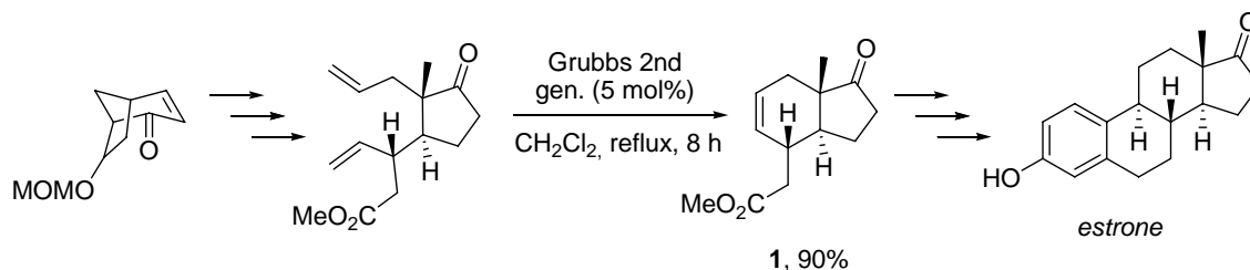
Scheme 5
