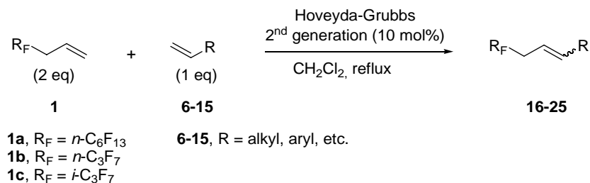
Scheme 27
