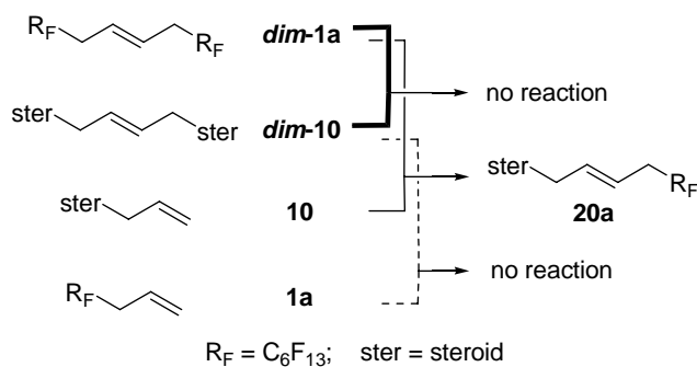
Scheme 29
