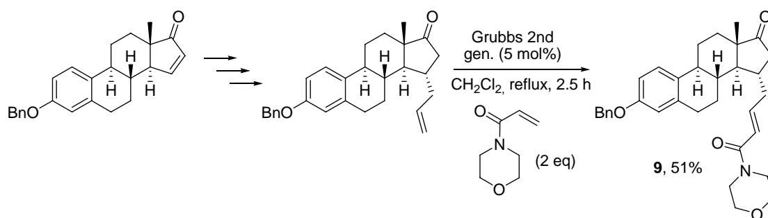
Scheme 12
