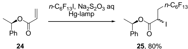
Scheme 18
