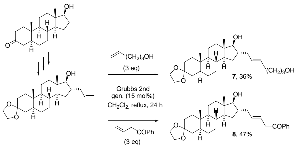
Scheme 11
