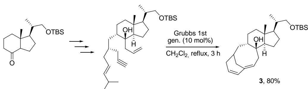
Scheme 7
