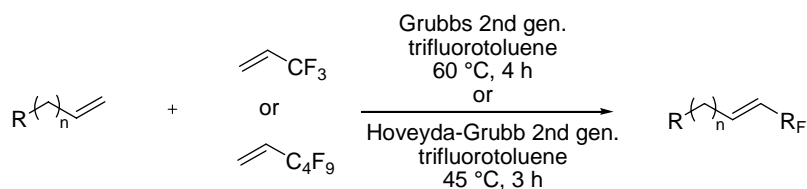
Scheme 24
