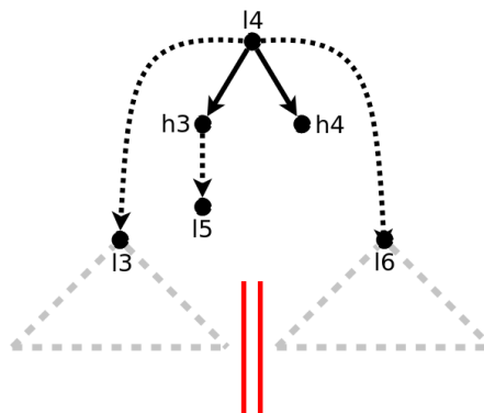
Figure 4.3: Ill-formed island fragment
