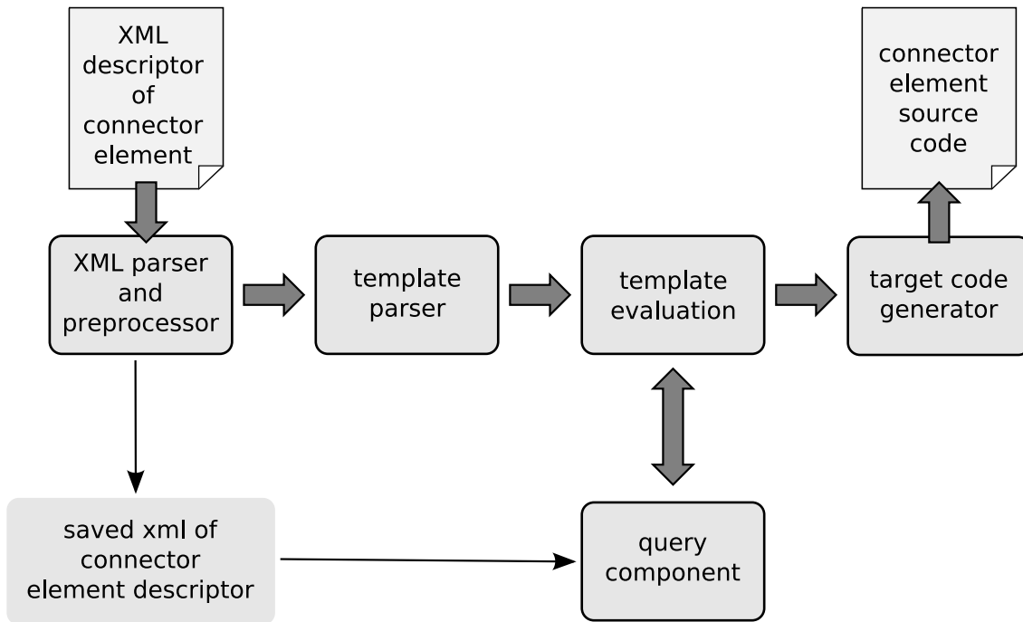
Figure 5.2: Stratego part architecture
