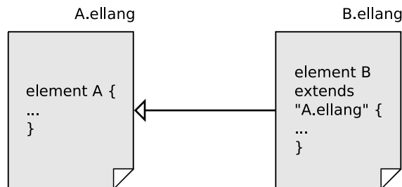
Figure 6.1: An example of template hierarchy
