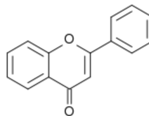
Fig. 11: Flavone
