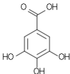
Fig. 10: Gallic acid
