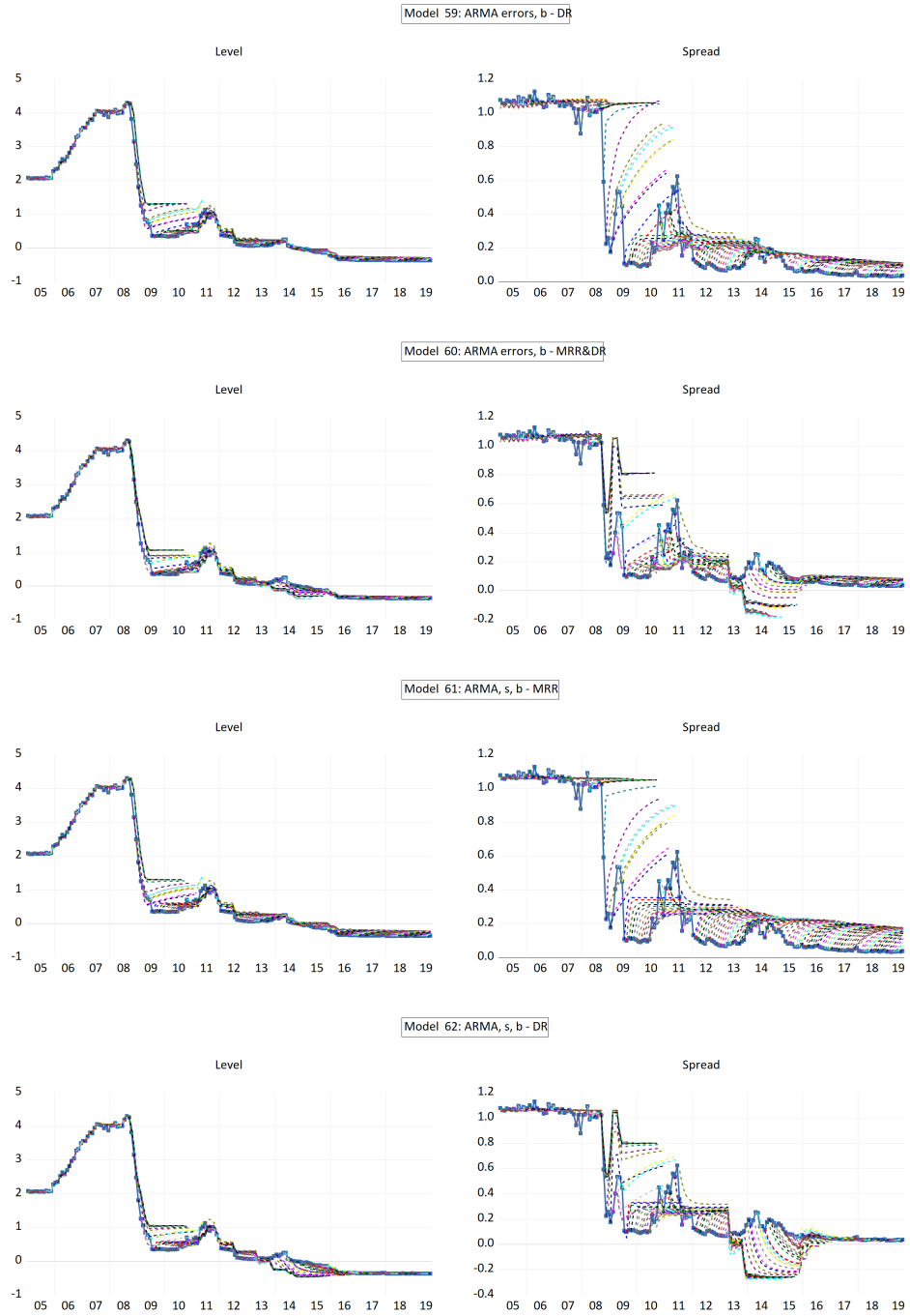
Figure 2.29: Eonia rate forecasts - Reduced-form models - Break (part 2)
