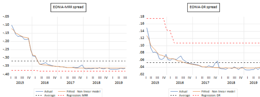
Figure 1.10: Model fit - Comparison with simple alternatives
