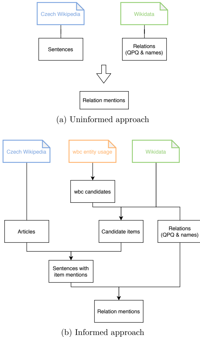
Figure 3.2: Diagrams contrasting the informed and uninformed approach of locating relation mentions in text.
