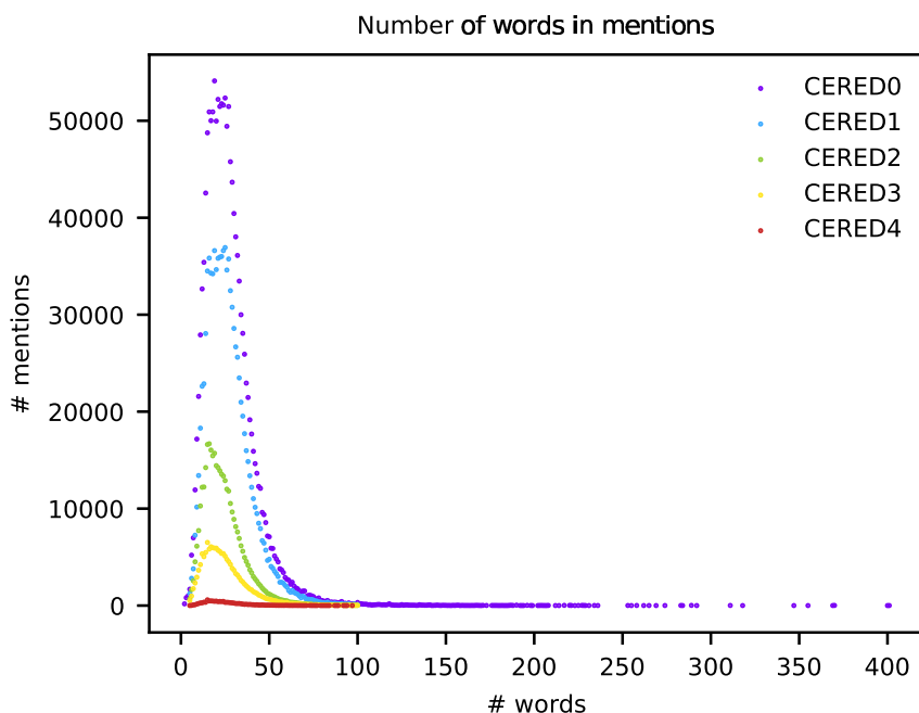
Figure 3.9: Histogram of mention lengths in words in CERED0-4.
