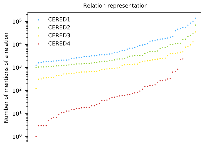
Figure 3.11: Number of mentions for different relation types in CERED datasets. For each dataset we ordered the relations by their frequency.
