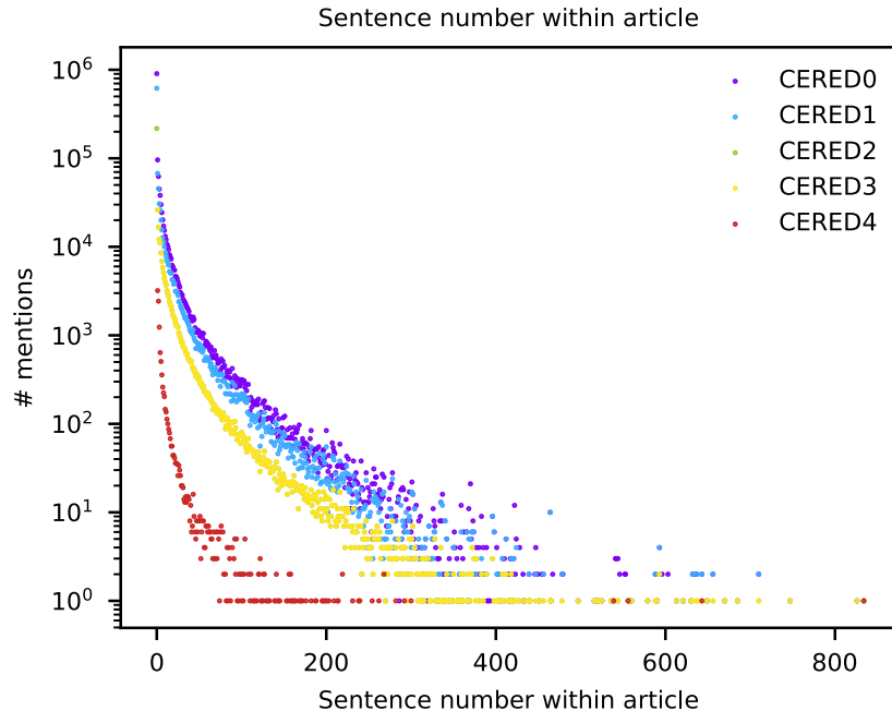
Figure 3.8: Distribution of the number of mentions for sentences with a given index in an article. In CERED0-2, first sentences dominate the datasets. CERED2 and CERED3 differ only in the first sentences, therefore CERED2 is mostly hidden by CERED3.
