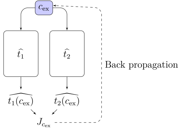
Figure 2.3: Network used for learning an extension defined by the equation t_1(x) = t_2(x) . \hat{t}_1 and \hat{t}_2 represent networks built based on the terms, just like in previous section. Note that only c_{\text{ex}} is optimized, everything else is treated as a function.
