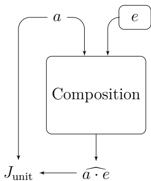
Figure 2.5: Learning of the unit. Learning is based on the axiom \forall a a \cdot e = a . The dual axiom e \cdot a had been disregarded for the sake of efficiency. The composition node represents the learned composition network.
