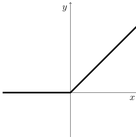
Figure 1.2: ReLU
