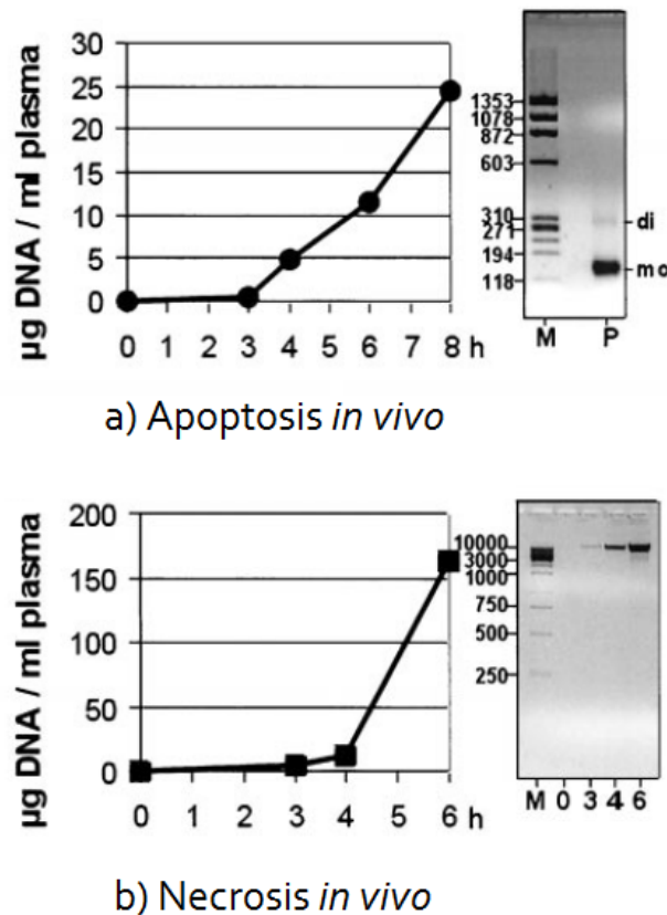
Figure 10. Demonstration of a rising DNA concentration in plasma after inducing cell death in mice. a) Apoptosis was induced with an injection of anti-CD95 antibody; visualisation exhibits apoptotic pattern with mono and di-nucleosomal fragments. b) Necrosis was induced with acetaminophen; long fragments characteristic for necrosis were observed. DNA concentration was analysed using qPCR (Jahr et al., 2001). di = dinucleosomal; mo = mononucleosomal fragments.
