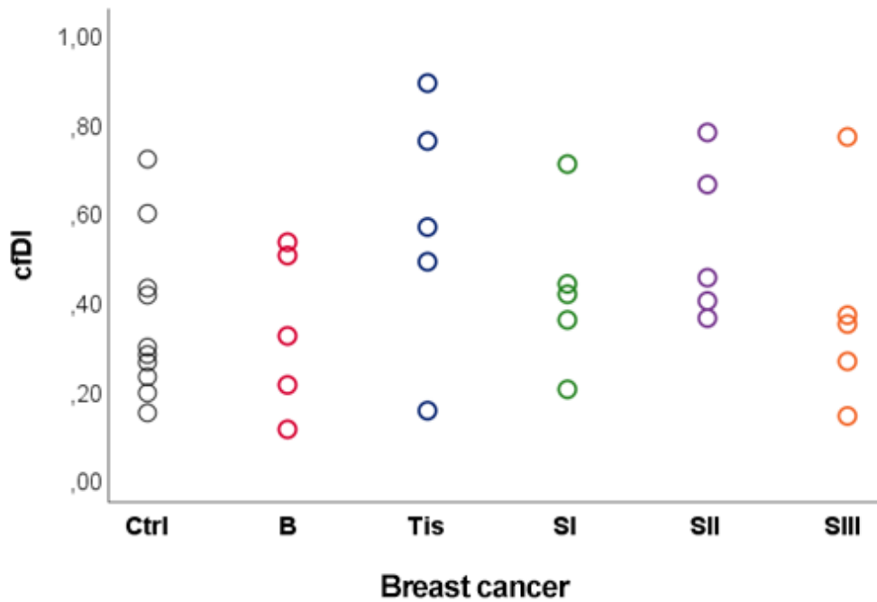
Figure 30. Scatter plot of cfDI in the breast carcinoma patients. Ctrl = controls; B = benign diagnoses; Tis = tumour in situ; S = Stage.
