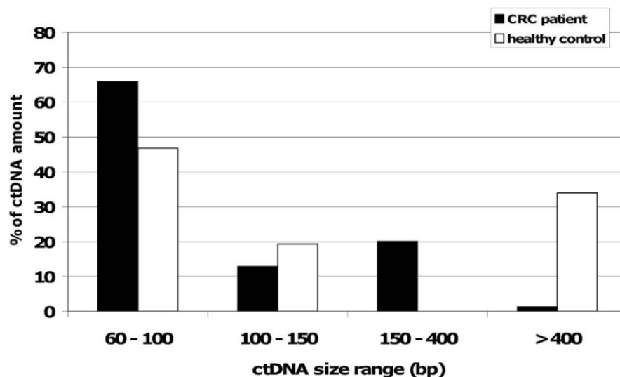
Figure 34. Amount of KRAS gene ctDNA amplicons categorized by size (Adapted from Mouliere et al., 2011).
