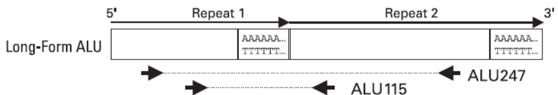
Figure 13. Annealing sites of Alu-based primers. Annealing sites of ALU-115 primers are situated within annealing sites for ALU-247, which ensures that ALU-115 amplify all the fragments, whereas ALU-247 only the longer ones (Adapted from Umetani et al., 2006).
