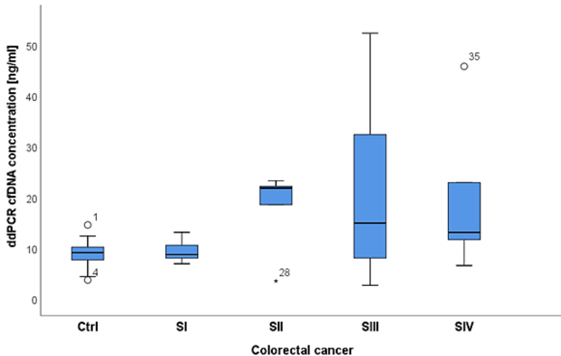
Figure 27. Boxplots with whisker-plots of cfDNA concentrations of individual stages in the colorectal cancer group compared to healthy controls. Boxes represent values within 25 – 75 percentiles with error bars and median. (○) = outliers; (*) = extreme outliers.
