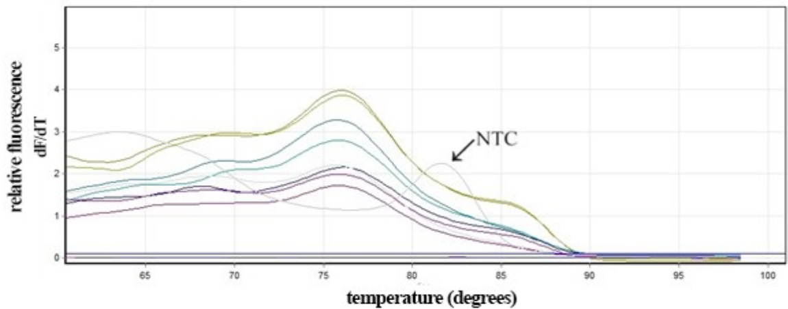
Figure 15. Melt curve analysis of reaction with test sample P464. The sample was isolated using both isolation kits. This reaction included P464 with and without added glycogen, ALU-115 primers were utilised, annealing temperature was 60°C.
