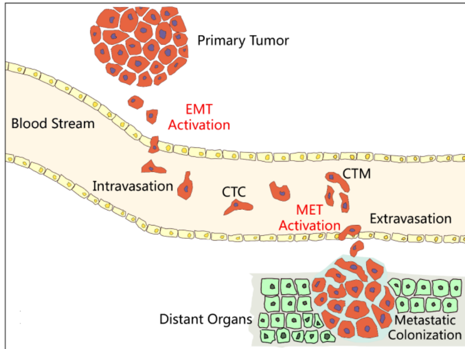
Figure 8. Scheme of emerging metastases. Tumour cells may undergo epithelial-mesenchymal transition (EMT), proceed into the blood and subsequently create new metastatic lesions through mesenchymal-epithelial transition (MET) (Adapted from Wu et al., 2017).
