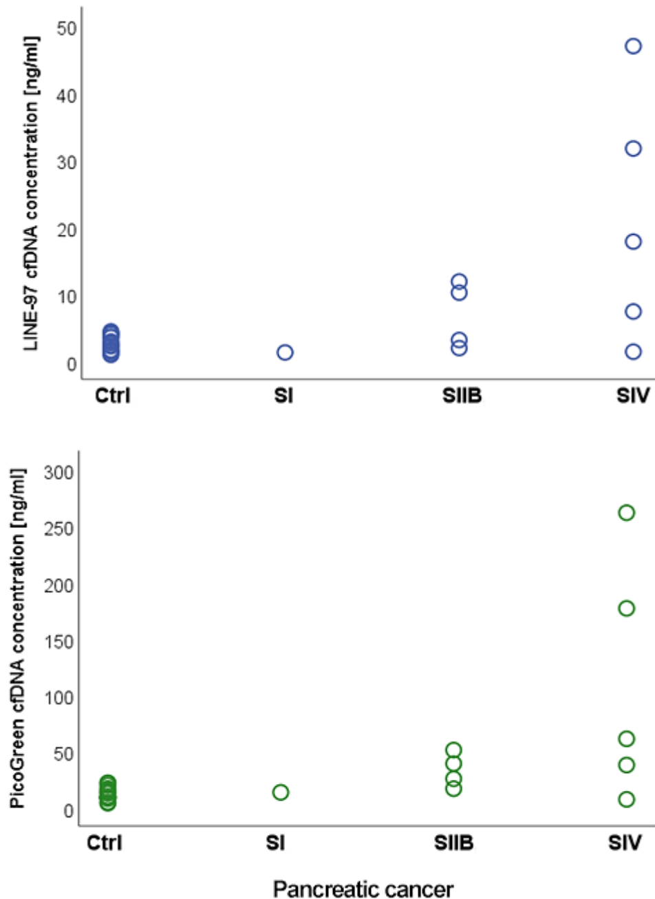
Figure 24. CfDNA concentration measured by qPCR using LINE-97 and PicoGreen assay in the pancreatic cancer group. Ctrl = healthy controls; S = Stage.
