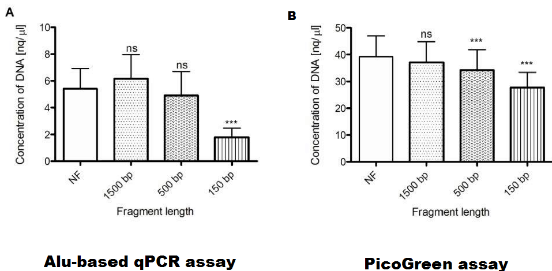
Figure 35. The DNA quantification of cfDNA using two different methods. (A) Alu-based qPCR assay with 10-fold diluted samples, (B) PicoGreen assay. DNA was fragmented into 1500bp, 500bp and 150bp fragments or was non-fragmented (NF) (Adapted from Sedlackova et al., 2013).
