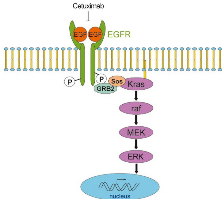
Figure 5. Scheme of Ras-Raf-MEK-ERK signalling pathway. Briefly described, epidermal growth factor (EGF), a ligand, binds to its receptor (EGFR) and activates its tyrosine-kinase activity, causing EGFR dimerisation and phosphorylation. After docking proteins (growth factor receptor-bound protein 2 - GRB2 and son of sevenless - SOS) are bound to phosphorylated EGFR, SOS exchange factor activates KRAS. Activated KRAS then activates BRAF kinase, which continues with activation and phosphorylation of MEK kinase, subsequently of ERK kinase, which in turn phosphorylates a transcription factor that regulates cell proliferation in the nucleus. If a patient is treated with an inhibitor of EGFR (cetuximab), treatment may be ineffective because of constitutively active Ras protein downstream of the signalling pathway (Edited and adapted from Wicki et al., 2010).
