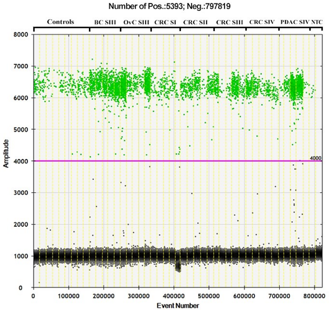
Figure 26. The number of positive (green) and negative (black) events. 5 393 of positive and 797 819 of negative droplets were observed.
