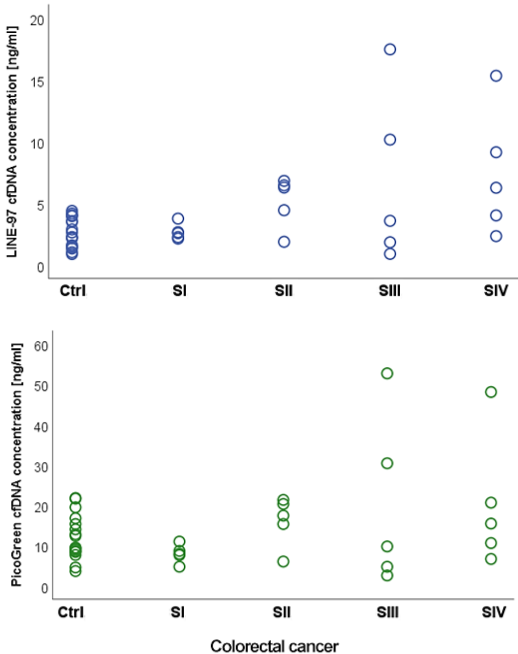
Figure 23. CfDNA concentration measured by qPCR by LINE-97 and PicoGreen assay in the colorectal cancer group. Ctrl = healthy controls; S = Stage.
