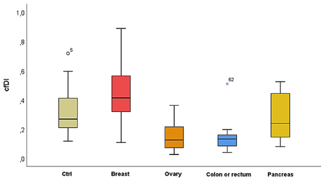
Figure 29. Boxplots with whisker-plots of cfDI in individual cancer groups. Boxes represent values within 25 – 75 percentiles with error bars and median. ( o ) = outliers; ( * ) = extreme outliers.
