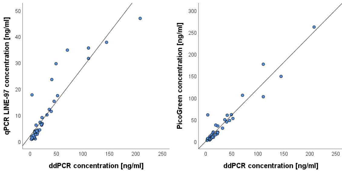
Figure 28. Linear regression curves for concentrations obtained by measurement methods. left: ddPCR and qPCR assay, right: ddPCR and PicoGreen assay.
