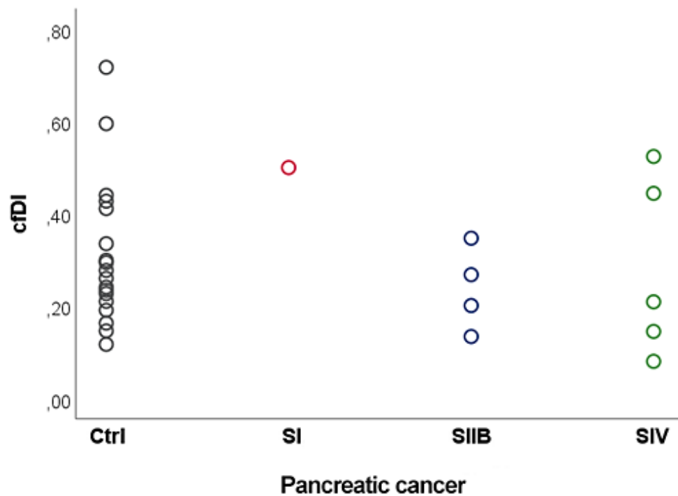
Figure 33. Scatter plot of cfDI in the pancreatic carcinoma group. Ctrl = controls; S = Stage.
