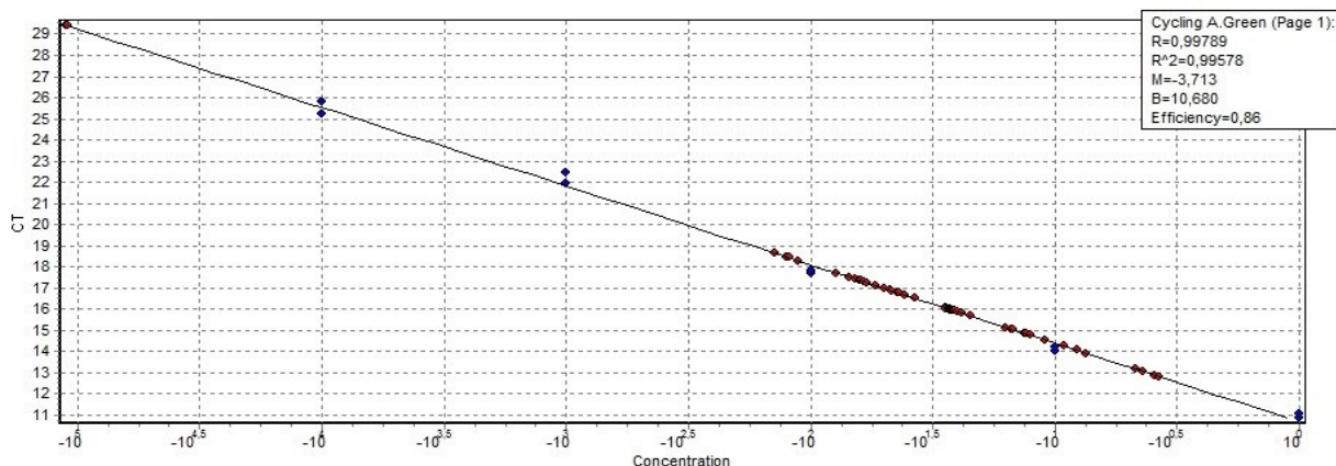
Figure 18. Points of the standard curve (blue dots). Samples P464, P470, P281, P282 of plasma and serum (red dots) using LINE-97 primers.
