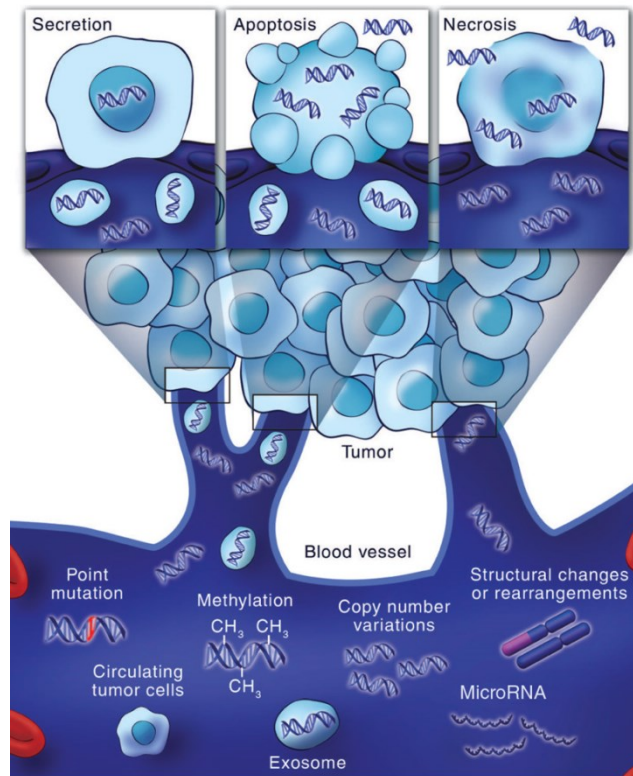
Figure 6. Scheme of various types of molecules, circulating tumour cells and exosomes present in the circulation of oncological patients (Adapted from Diaz and Bardelli, 2014).
