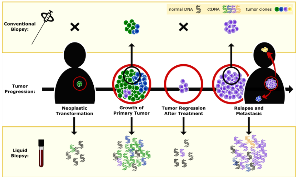
Figure 7. Representation of overcoming the limitation by using liquid biopsy compared to conventional biopsy (Adapted from www.genengnews.com/uncategorized/gen-roundup-liquid-biopsies-remain-wait-and-see-for-some-clinicians ).
