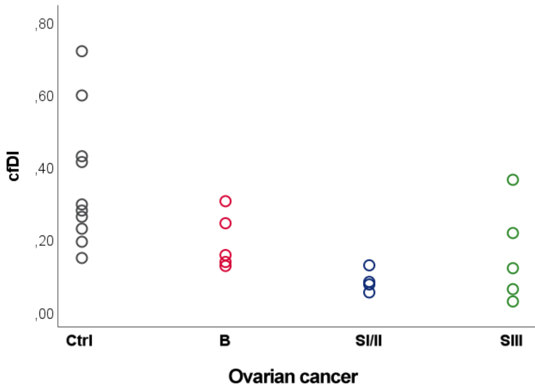
Figure 31. Scatter plot of cfDI in the ovarian carcinoma group. Ctrl = controls; B = benign diagnoses; S = Stage.
