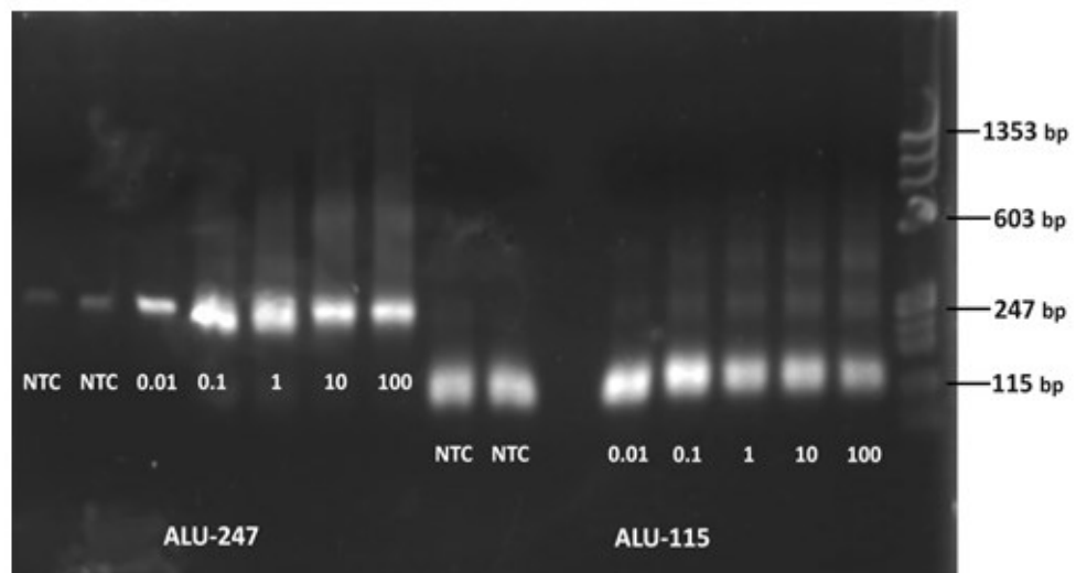
Figure 16. Products of qPCR reaction using ALU-115 and ALU-247 primers. Standard DNA of concentrations 100 – 0.01 pg/rxn (40 – 0.04 pg/μl), described below each sample. Amplification products were present in all non-template controls.
