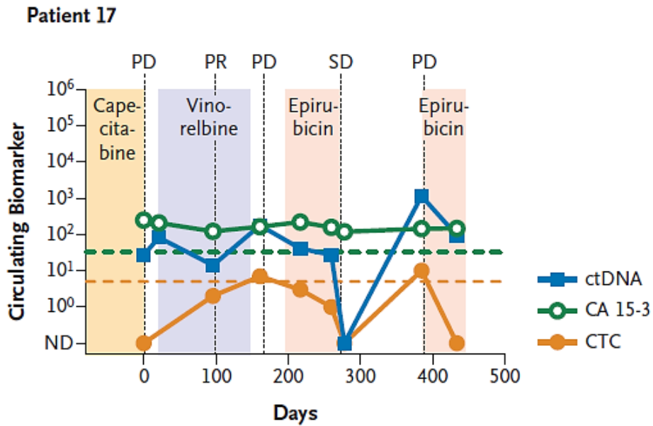
Figure 12. Changing levels of ctDNA, tumour marker CA15-3 and CTCs in patients suffering from metastatic breast cancer. The level of ctDNA after ended epirubicin treatment has risen, which indicates the progress of the disease. SD = stable disease; PR = partial response; PD = progressive disease. ctDNA is shown as a number of copies/ml of plasma; Orange line represents 5 CTCs/7.5ml of blood; green lines represent the threshold of CA15-3 32.4 U /ml (Adapted from Dawson et al., 2013).
