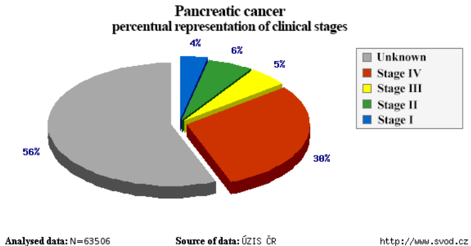
Figure 3. Incidence of individual stages of pancreatic cancer. Clinical data are established based on TNM classification valid at the time of diagnosis (Adapted from ÚZIS ČR).
