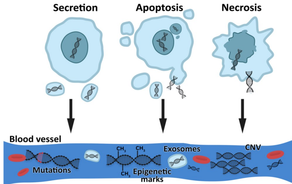
Figure 9. Scheme of origin and properties of cfDNA. CfDNA provides real-time information about patient's condition by monitoring cfDNA concentration, integrity, specific mutations, copy number variations (CNV), epigenetic marks, loss of heterozygosity etc.
