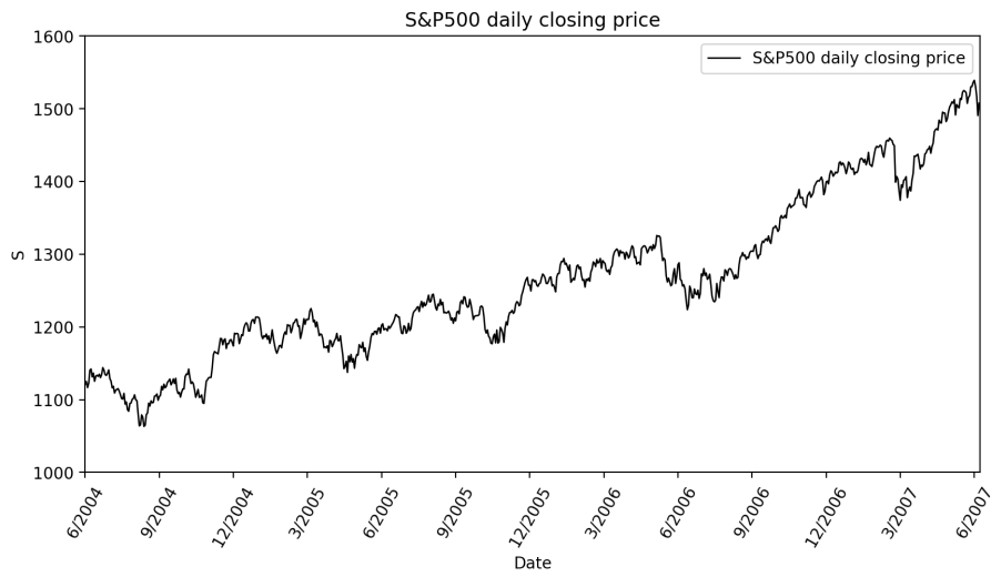
(a) S&amp;P500 daily closing prices between 2004-2007
