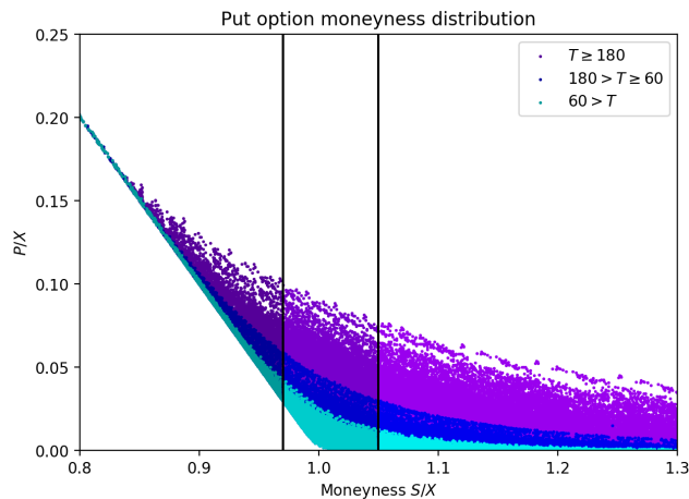
(b) Put options
