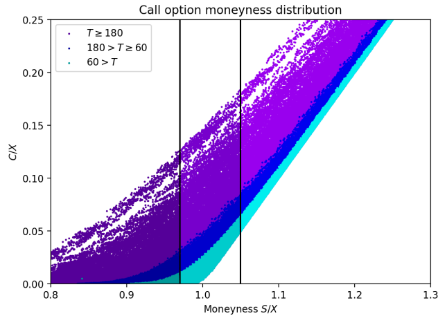
(a) Call options
