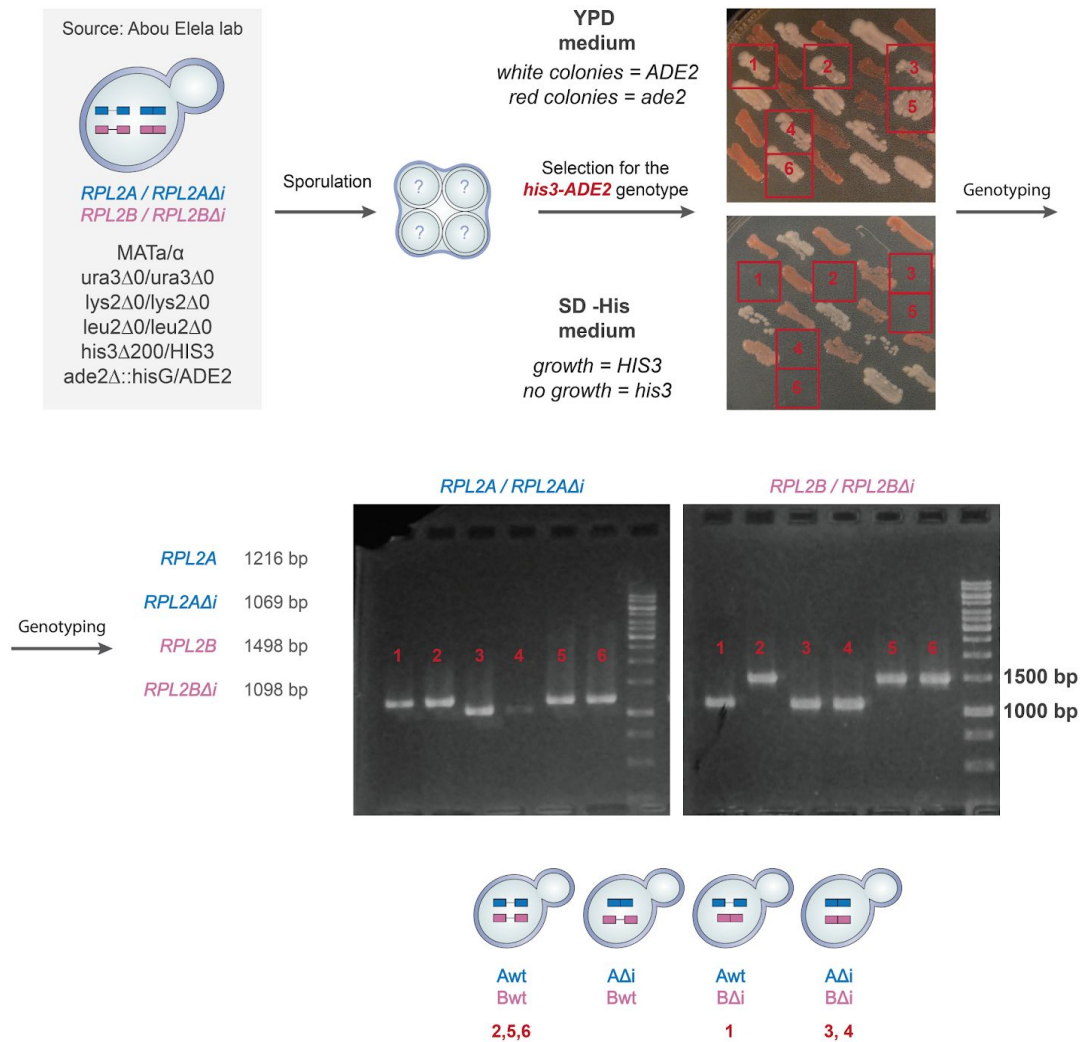
[Supplementary Figure 1] Strategy to create haploid strains used for testing of candidate RP genes. Shown is the example of preparation of RPL2 strains. Diploid strains containing heterozygous intron deletion ( \Delta i ) in each RPL2 paralog, kindly provided from Abou Elela lab, were sporulated and haploid cells selected for the presence of his3-ADE2 (we also selected for the HIS3-ade2 ) auxotrophic markers (to allow for subsequent experiments). Intron deletion was confirmed by PCR genotyping, in the case of RPL2 paralogs by using KA114-115 ( RPL2A ) and KA116-117 ( RPL2B ) primers. Genotyping of 6 independent colonies identified Awt/Bwt, Awt/B \Delta i and A \Delta i /B \Delta i strains. Overall, we prepared 3 independent strains for each genotype.
