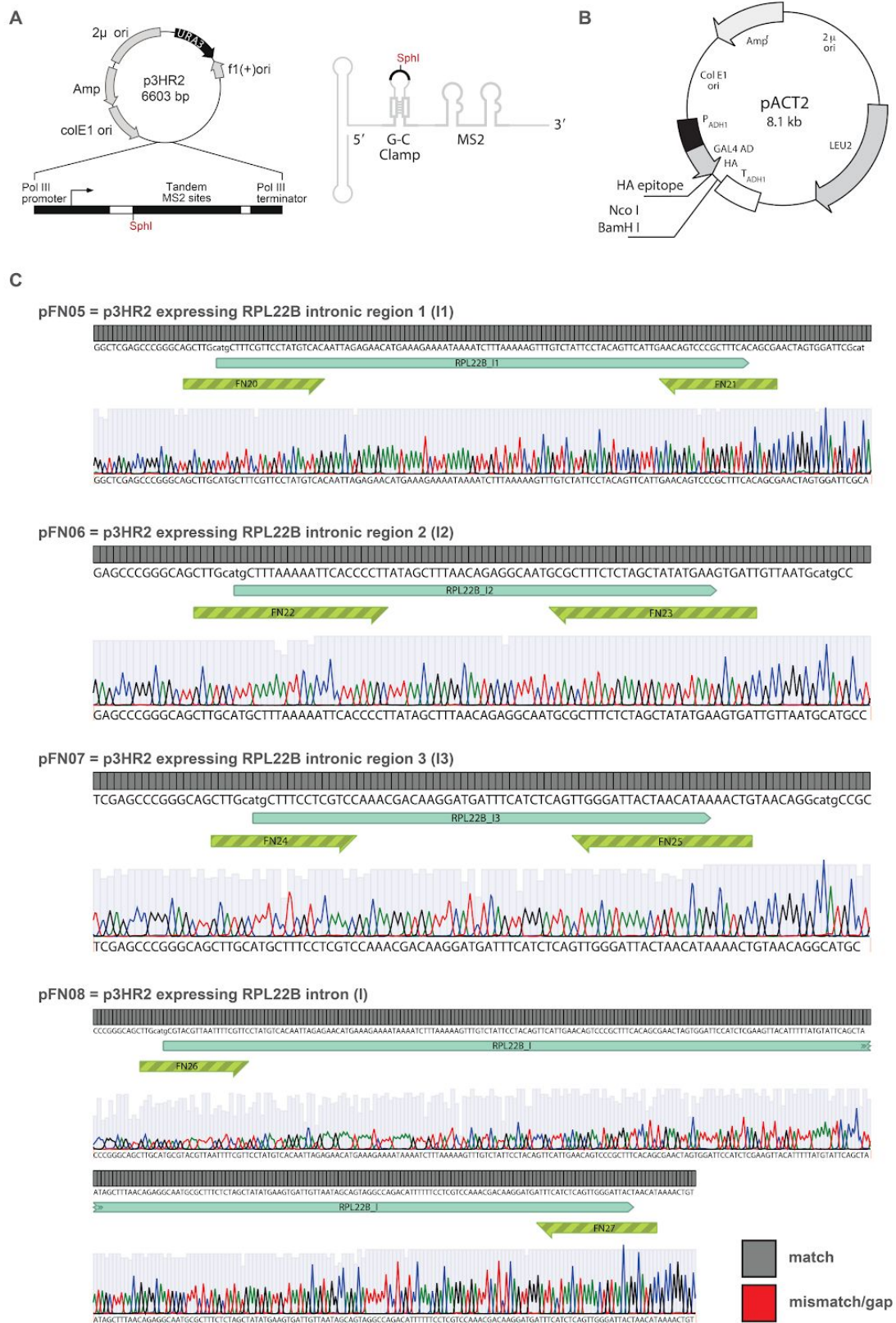
[Supplementary Figure 2] S.cerevisiae constructs used in the 3-H system. (A) Map of the p3HR2 plasmid showing the region ( PaeI site), where the RNA of interest was cloned. (B) Map of the pACT2 plasmid. (C) Alignment (Benchling) showing the correctness of RNA constructs used in the study.
