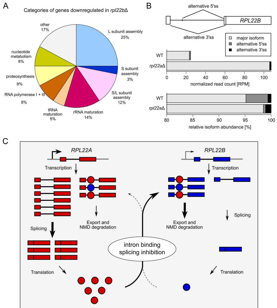
Fig 8. Intergenically regulated RPL22 paralogs may have differentiated roles. (A) Deletion of RPL22B has little effect on total RPL22 levels but affects a subset of genes involved in ribosome biogenesis and proteosynthesis. (B) The scheme depicts alternative splice sites used in RPL22B pre-mRNA splicing. The upper plot shows read counts for each spliced RPL22B product, normalized to sequencing library sizes (RPM, reads per million). The lower plot shows
