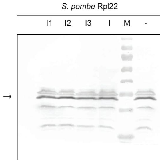
[Supplementary Figure 3] Interactions of Rpl22 orthologs with the RPL22B intron. (A) Interactions assayed using yeast 3-H system with the HIS3 reporter. Cells were spotted in 10-fold serial dilutions on plates without His (-U-L-H) or additionally in the presence of 3-aminotriazole (3-AT). Shown are representative plates from at least three independent experiments. (B) Western blot analysis with anti-HA antibody against HA-tagged Gal4 activation domain. Hybrid protein of 31 kDa (marked with an arrow) was detected in extracts of strains with all tested constructs. M - protein size marker PageRuler™ Plus Prestained Protein Ladder (Thermo Scientific).
