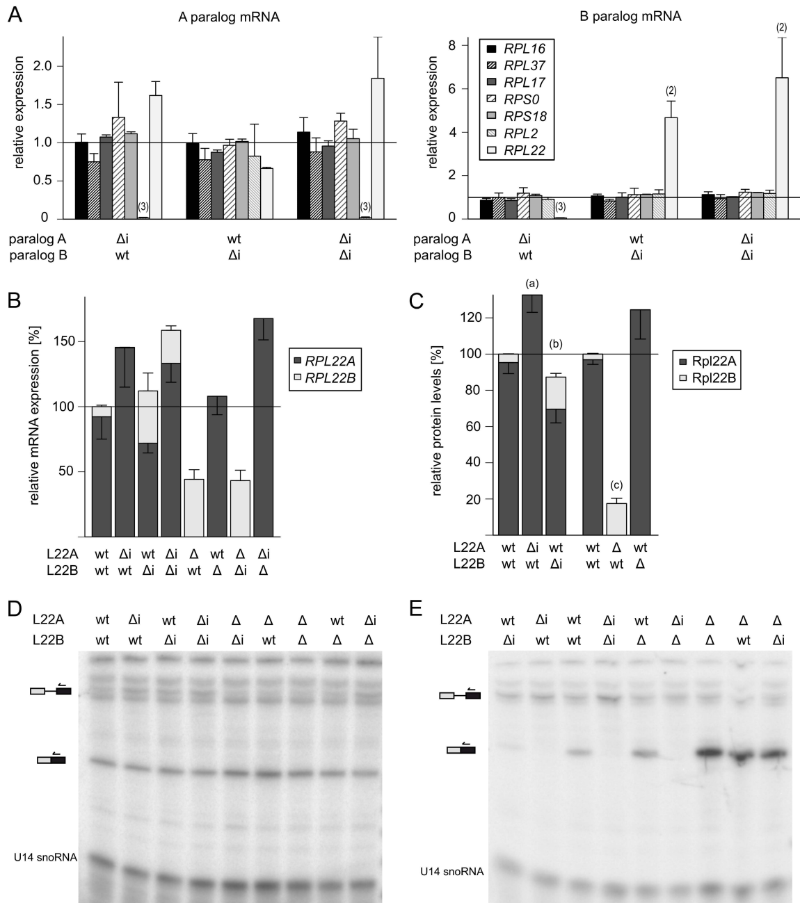
Fig 1. Introns mediate intergenic regulation of RPL22 paralogs. (A) Impact of intron deletions on the expression of duplicated ribosomal protein genes. Transcript levels of RPL16, RPL17, RPL37, RPS0 and RPS18 paralogs are refractory to intron deletions. In contrast, RPL22 and RPL2A show intergenic
