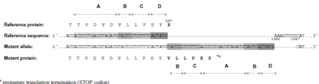
Fig. 1. Heterozygous microindel mutation in exon 4 of TRPS1 gene (c.1940_1947del8ins39; p.E647Vfs*5), shift of the reading frame and stop codon position. Reference sequence is following the transcript 1 mRNA nucleotide and amino acid position (NM_0141124).
