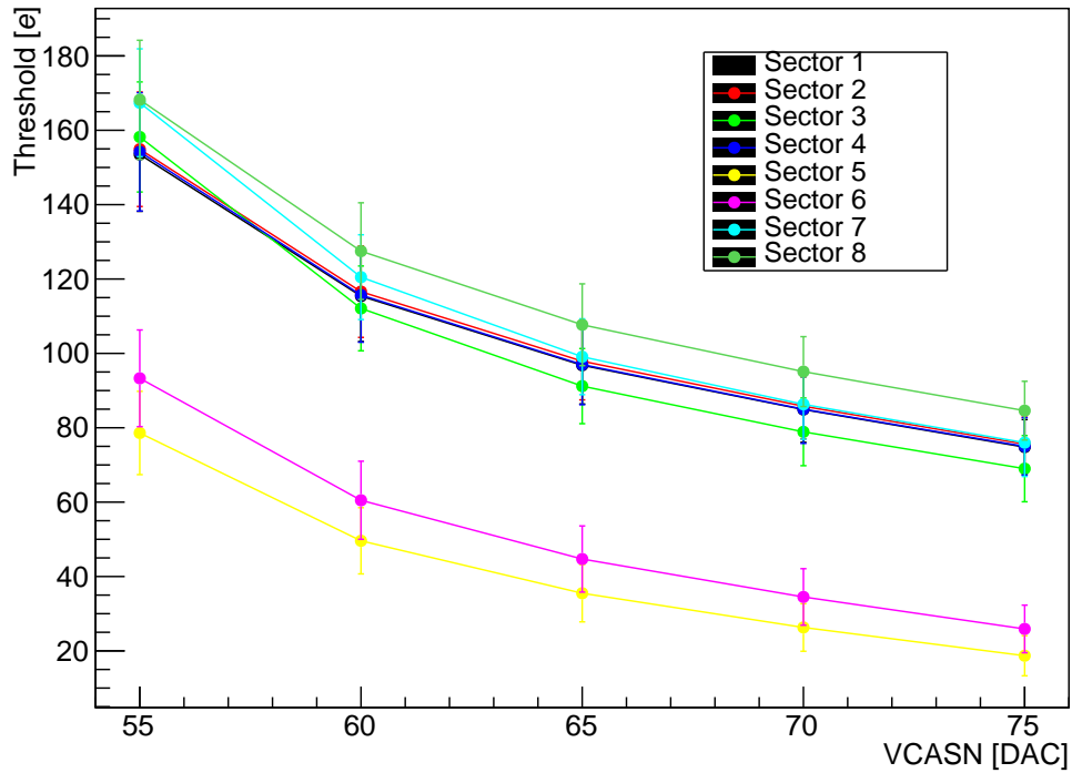
Figure 3.9: Mean threshold as a function of VCASN for ITHR = 60 for each of the 8 sectors of the pALPIDEfs-3 chip.
