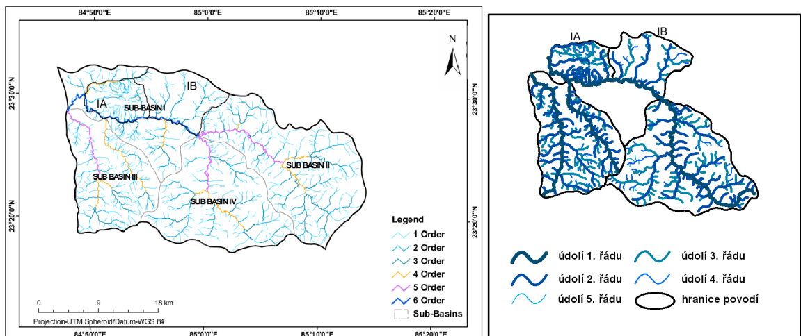
Figure 3. Drainage and sub basin map of study area.
