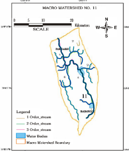
Figure 16: Drainage Classification of Macro Watershed No. 11
