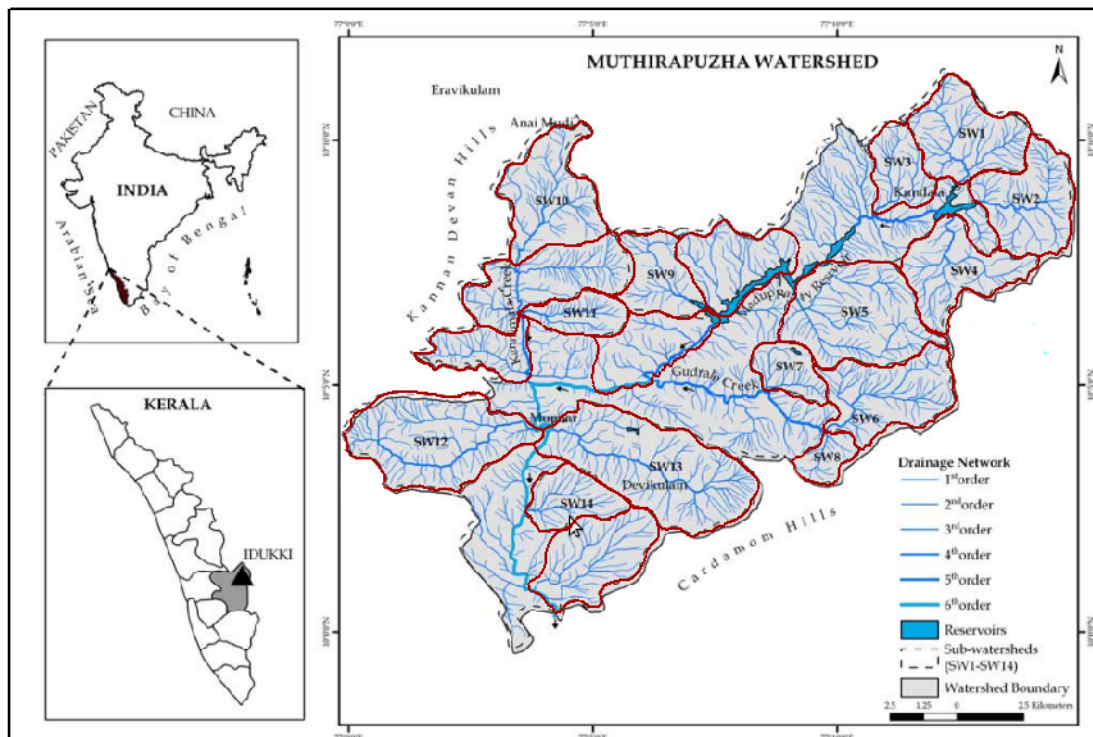
Figure 1. Muthirapuzha watershed (MW) and fourth order sub-watersheds.
