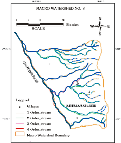
Figure 8: Drainage Classification of Macro Watershed No. 3.
