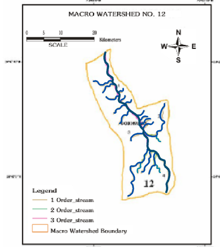
Figure 17: Drainage Classification of Macro Watershed No. 12
