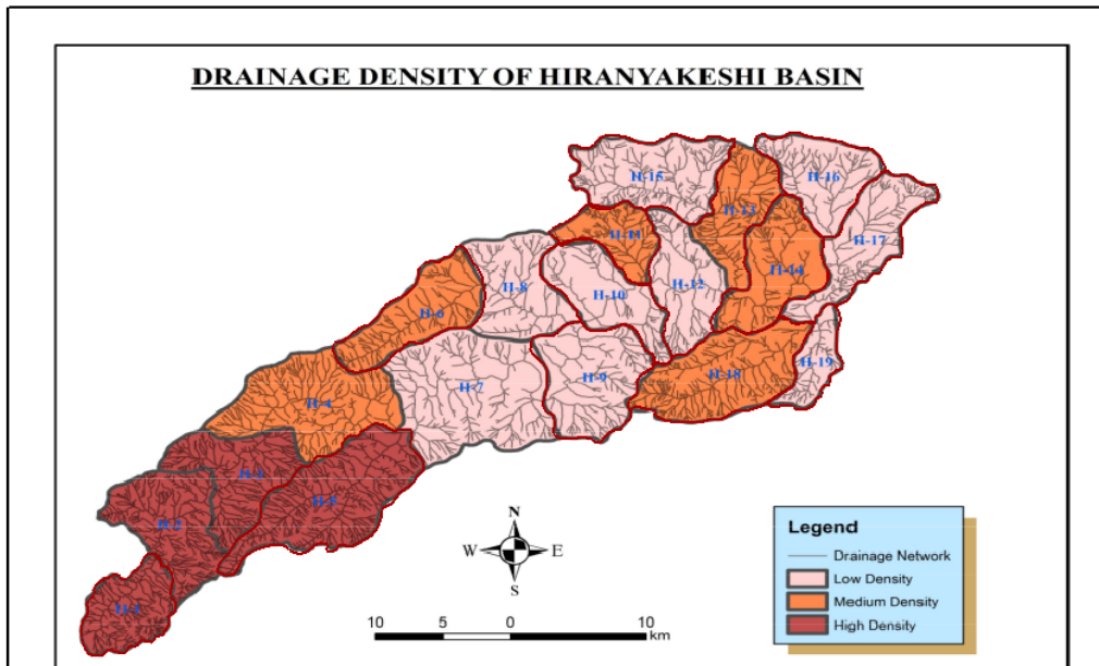
Figure 5: Drainage density of Sub-Basins
