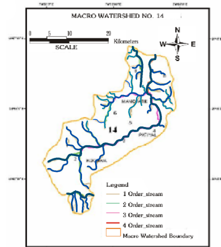
Figure 19: Drainage Classification of Macro Watershed No. 14
