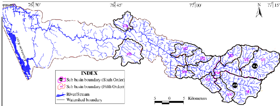
Fig.1. Drainage network map of Achankovil river basin
