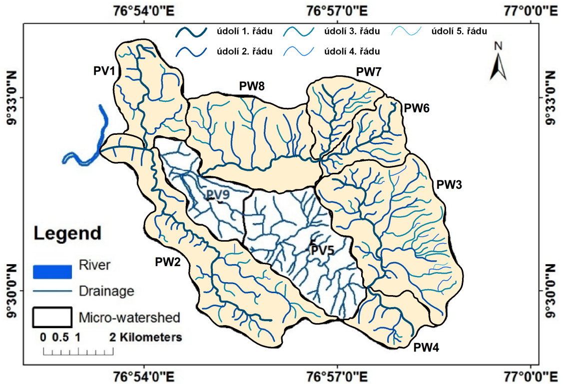
Fig.2 Map showing micro-watersheds of Peruvanathanam sub-watershed
