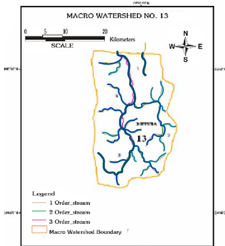
Figure 18: Drainage Classification of Macro Watershed No. 13
