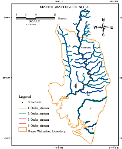
Figure 9: Drainage Classification of Macro Watershed No. 4.
