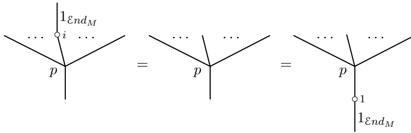
Figure 1.3: Unit axiom p \circ_i 1_{\mathcal{E}nd_M} = p = 1_{\mathcal{E}nd_M} \circ_1 p .
