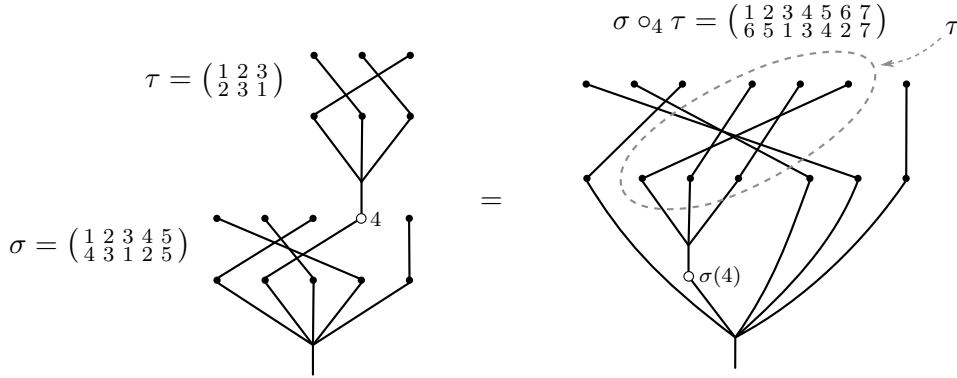
(b) Equivariance – (p_k\sigma) \circ_i (q_l\tau) = (p_l \circ_{\sigma(i)} q_l)[\sigma \circ_i \tau] .
