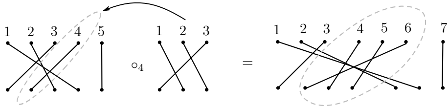
Figure 1.6: \circ_i for permutations.
