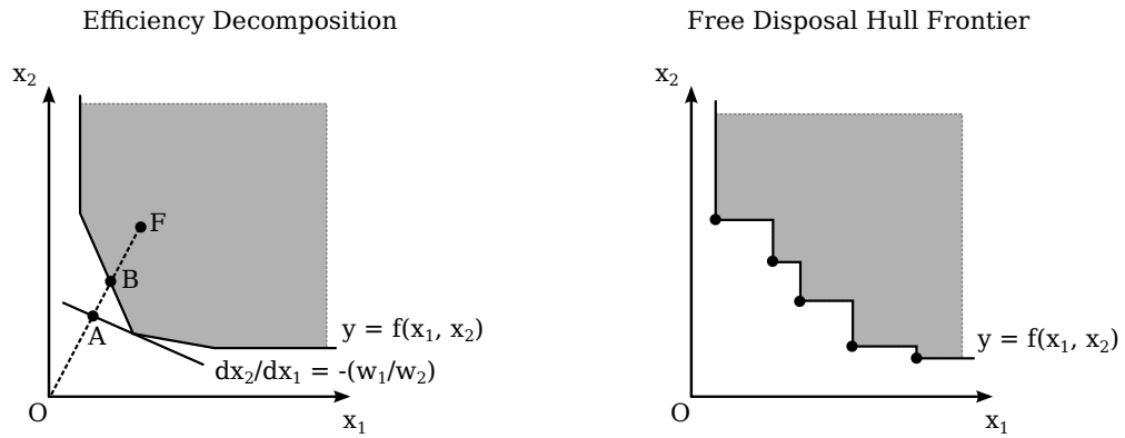
Figure 2.1: Efficiency decomposition and Free Disposal Hull frontier.
