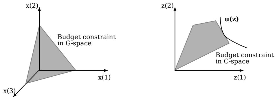
Figure 2.2: An illustrative transformation of budget constraint from \mathcal{G} -space to \mathcal{C} -space
