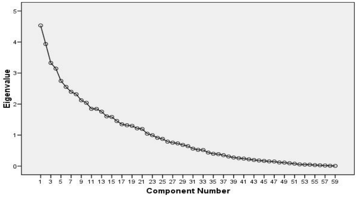
Scree Plot
