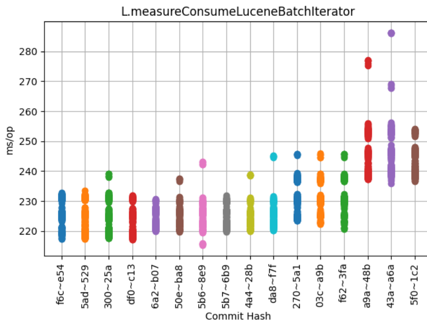
Obrázek 6.6: L.measureConsumeLuceneBatchIterator
