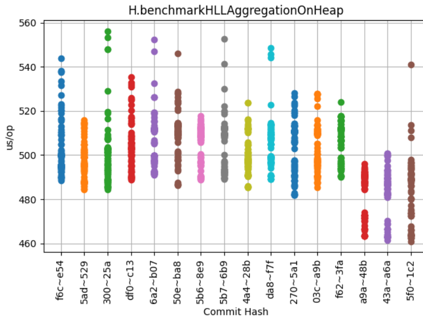
Obrázek 6.34: H.benchmarkHLLAggregationOnHeap
