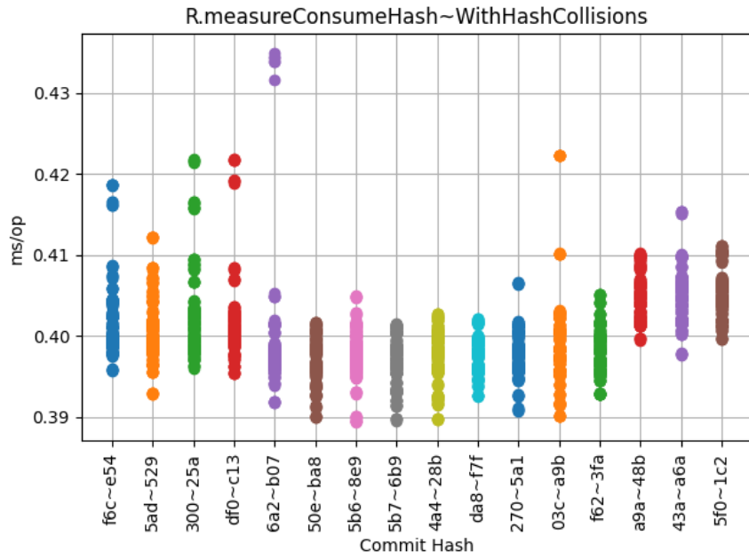
Obrázek 6.13: R.measureConsumeHash~WithHashCollisions
