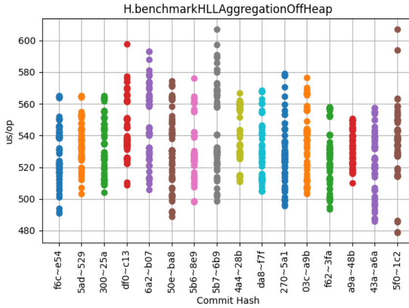
Obrázek 6.33: H.benchmarkHLLAggregationOffHeap
