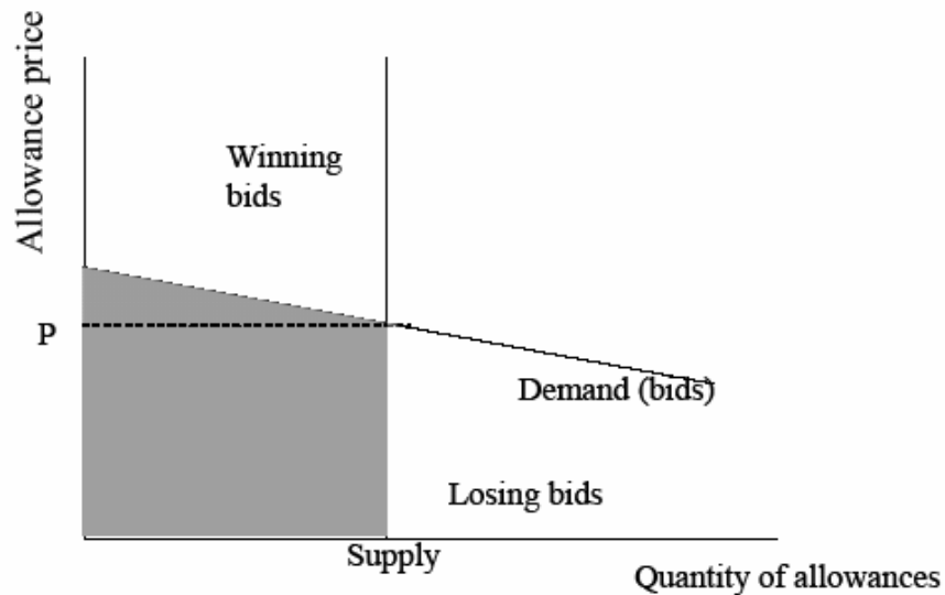
Figure 9 : Pay-your-bid Auction
