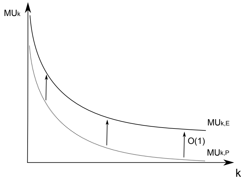
Figure 3.2: Marginal utility of child adoption under Extended Family setting
