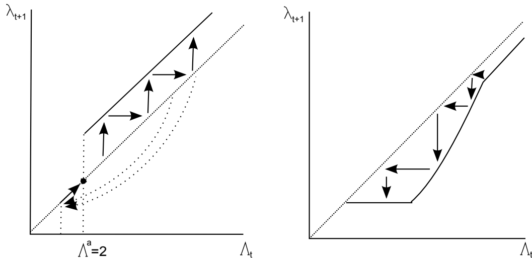
Figure 3.3: Human Capital Accumulation - Extreme Cases
