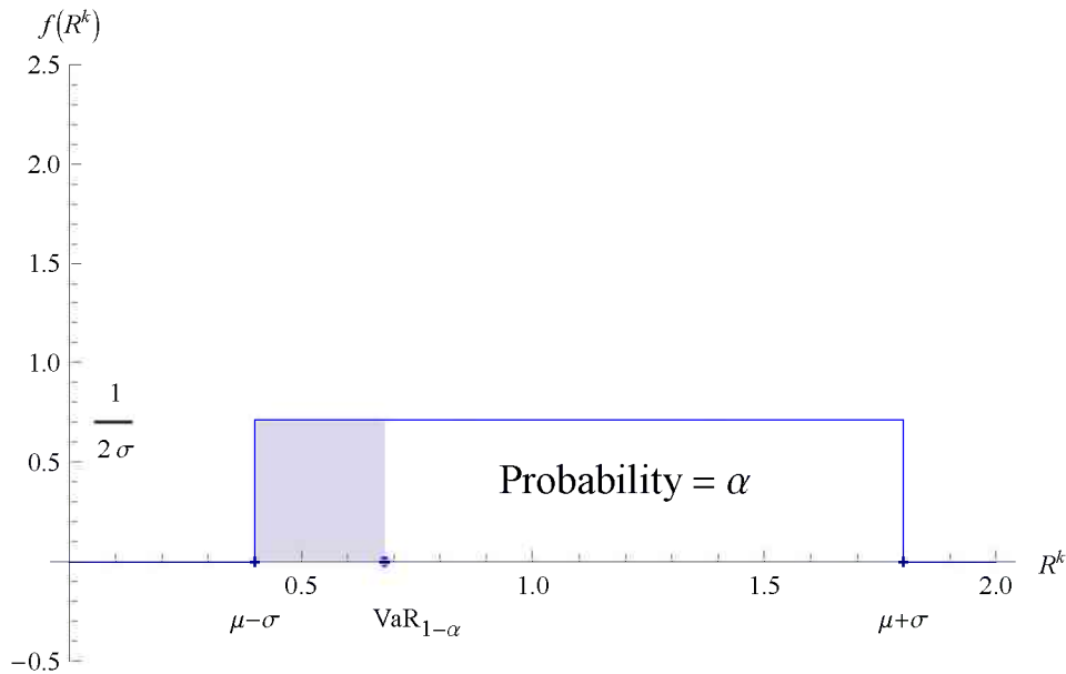
Figure 2.1: VaR of uniformly distributed return on capital
