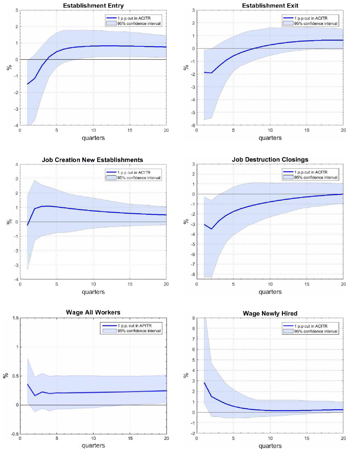
Figure 3.2: Impulse Responses: Augmented VAR Model
