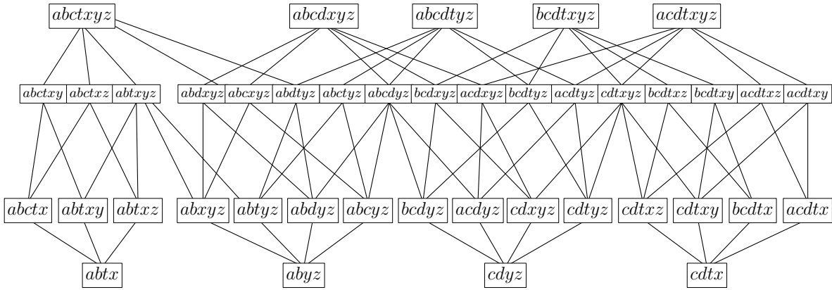
Figure 3.13. Sets G with w'(G) \neq w'(H)
