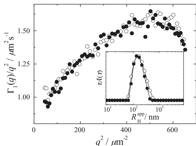
Fig. 3. Dynamic Zimm plots for Cel-g-PS-I (solid circles) and Cel-g-PS-II (open circles) in aqueous dispersions. Insert: CONTIN distributions of apparent hydrodynamic radii for Cel-g-PS-I (solid circles) and Cel-g-PS-II (open circles) at the scattering angle \theta = 90^\circ .
