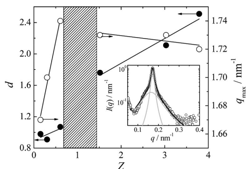
Figure 6. Power law exponent, d , and position of the maximum of the correlation peak, q_{\max} , as functions of Z . Precipitation region is shown as hatched area. Inset: The SAXS scattering peak for Z = 3.79 and its fit by the sum of two Lorentzian functions.
