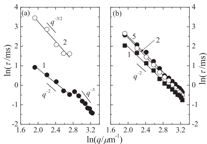
Fig. 5. Mean relaxation times of the modes observed in CONTIN distributions of (a) oleate-SPION dispersions ( c_{NP} = 1 \text{ g l}^{-1} ): curve 1 – fast mode, curve 2 – slow mode and (b) QNPHOS-PEO/oleate dispersions ( c_{NP} = 1 \text{ g l}^{-1} ) at various c_P (indicated above the curves in \text{g l}^{-1} ).
