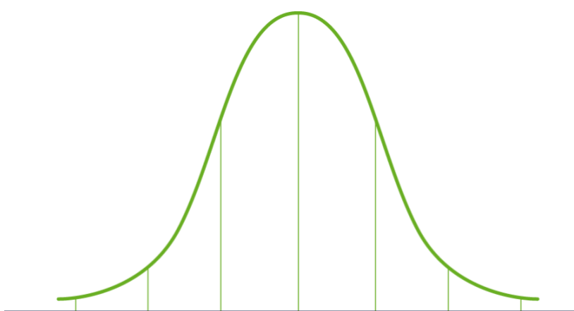
Figure 13. Normal distribution.
