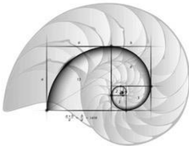
Figure 17. Nautilus shell and Fibonacci sequence.
