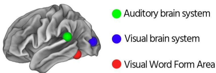
Figure 1. Visual word form area and other connected areas critical for reading.
