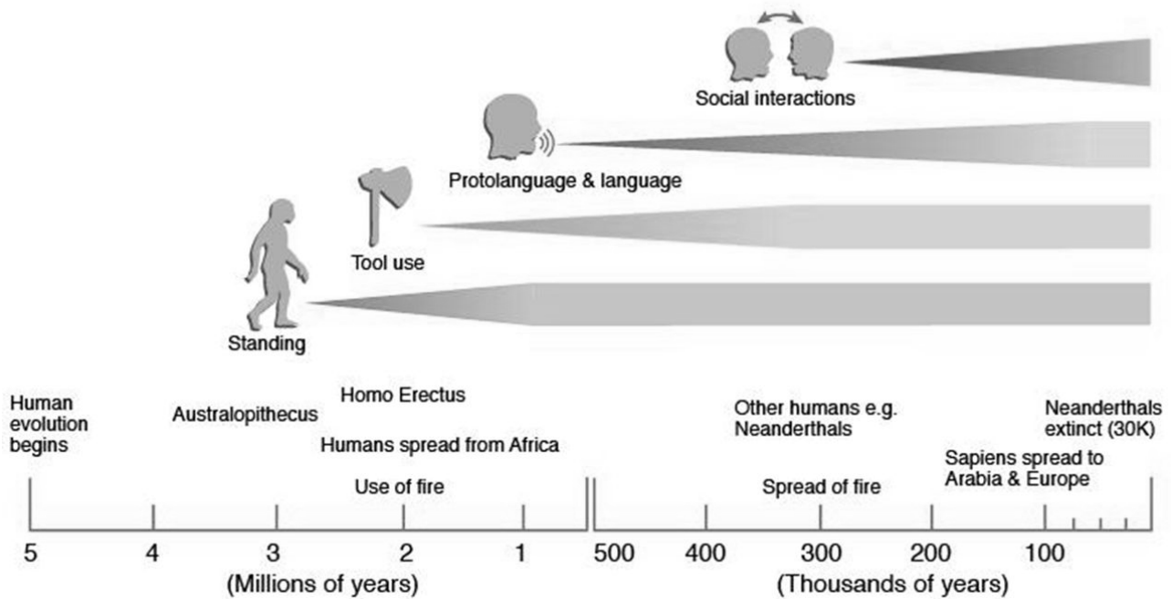
Figure 22. Fundamental steps in human evolution.
