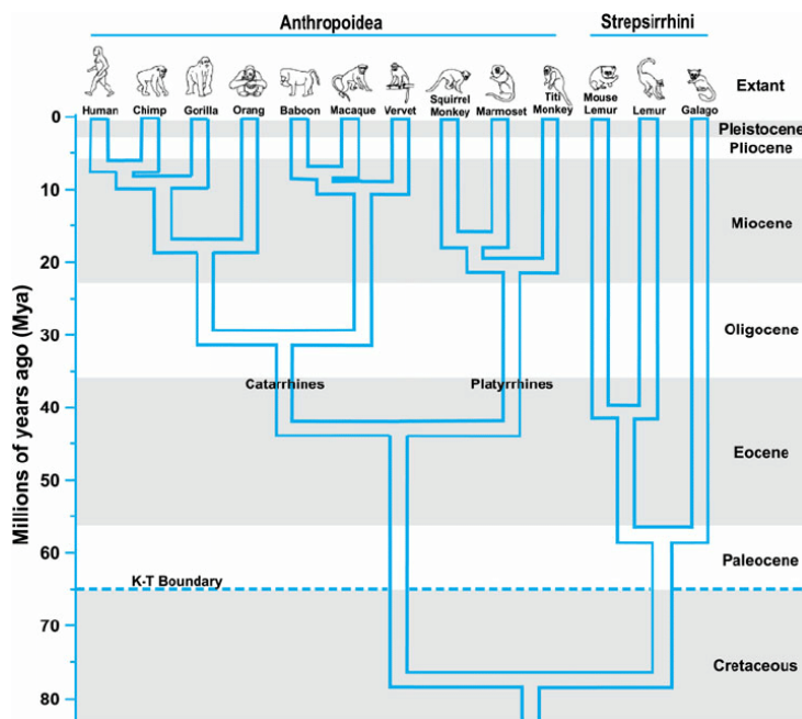
Figure 12. Phylogenesis of the major primate groups
